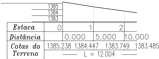
PERF "D"
